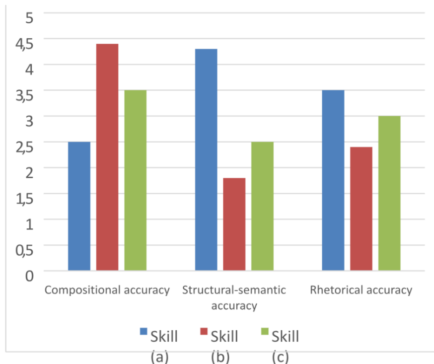
Figure 2. Statistics result
